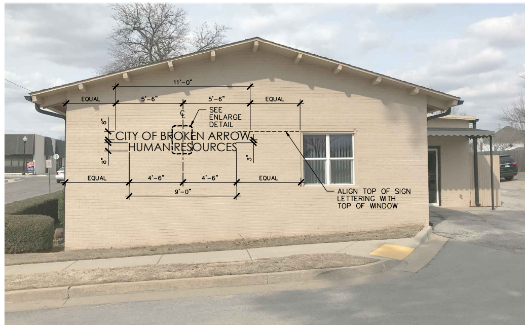
C ELEVATION: SIGNAGE C NOT TO SCALE
